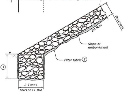
FIGURE 5 ~ PROTECTION STONE RIPRAP ⑤
