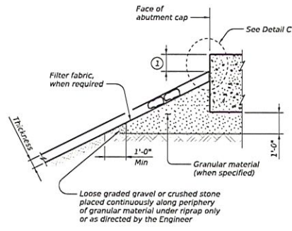
SECTION A-A AT CAP
