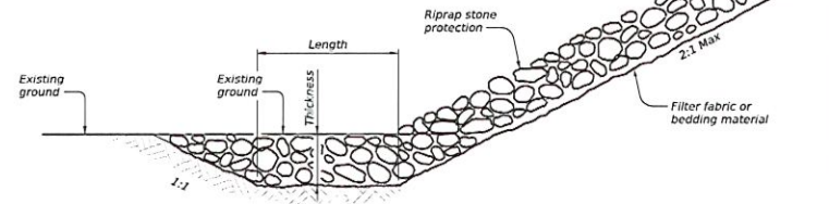
EXTENDED ROCK FILLED TRENCH
