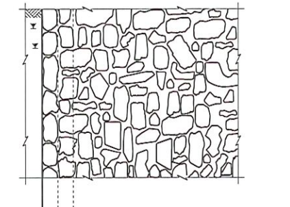
FIGURE 1 ~ TYPE R STONE RIPRAP Dry or grouted
