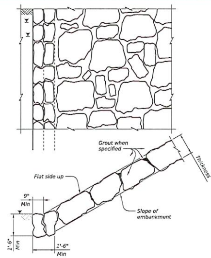
FIGURE 3 ~ TYPE F STONE RIPRAP Grouted
